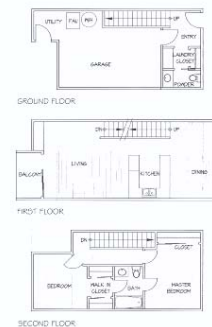
TOWNHOUSE PLANS
